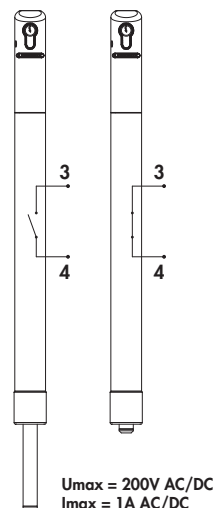
Optional dropbolt position detection
